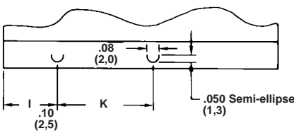
“D” Lance Detail
