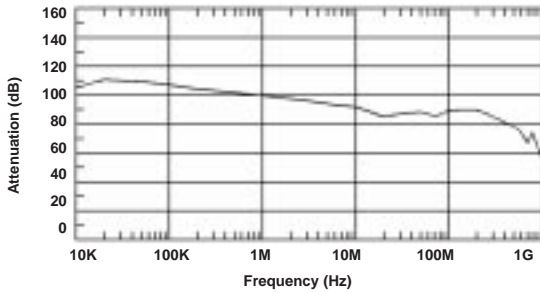
Shielding Effectiveness Transfer Impedance Test 97-654
