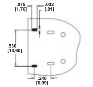
Top View: Minimum Protrusion PCB Layout
