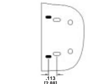
Top View: Maximum Protrusion PCB Layout
