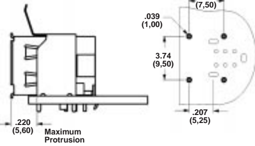
Printed Circuit Board Layout
