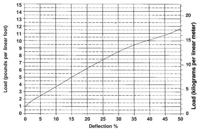
Compression - Deflection Part No. 8417-3052-62
