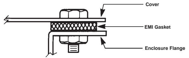
Figure 4. Flat Gasket between Sheet Metal Flange
