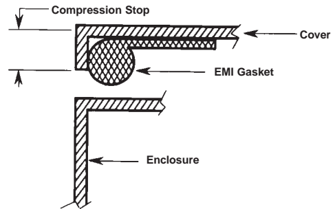
Figure 5a. Cover with Compression Stop
