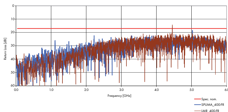
Return loss vs. frequency (SPUMA_400-FR vs. LMR_400-FR)
