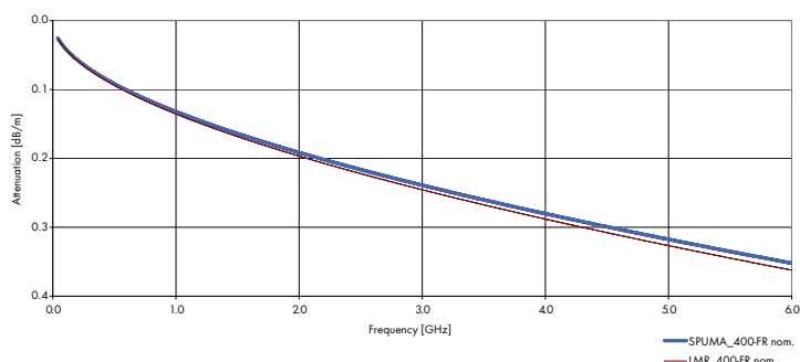
Attenuation vs. frequency (typical) (SPUMA_400-FR vs. LMR_400-FR)
